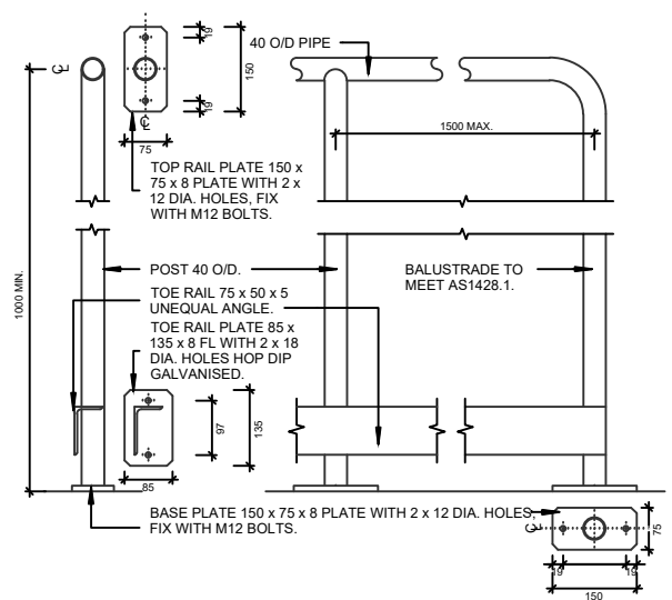
3 RAMP DETAIL SECTION NOT TO SCALE
