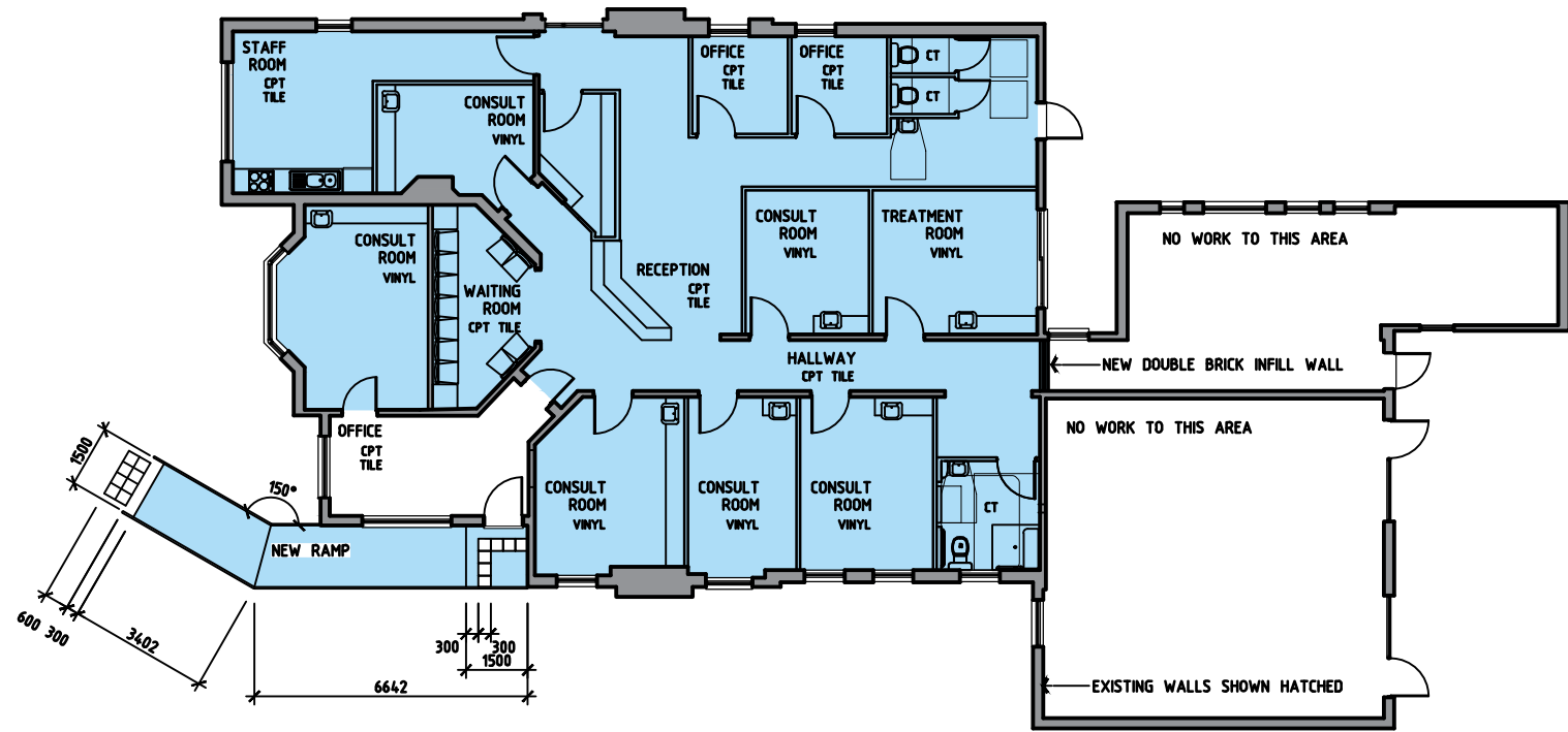
1 RAMP DETAIL PLAN 1:100 @ A1 SHEET SIZE
