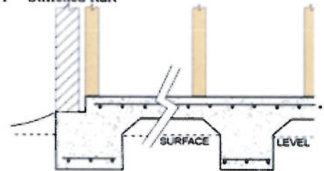
Fig. 1 Stiffened Raft
