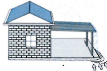
Fig. 10 Soil Drainage Plan
